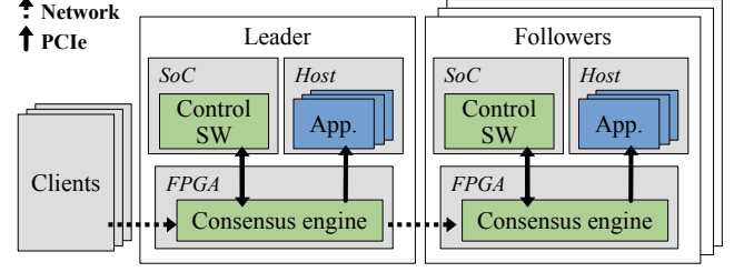
Figure 1: Nano-consensus architecture across multiple nodes.
