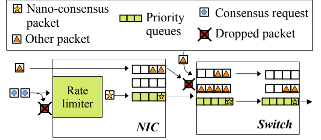
Figure 3: Nano-consensus sample communication in a section of the network. Consensus requests from clients and other packets can be dropped while Nano-consensus makes its packets never exceed network capacity.
